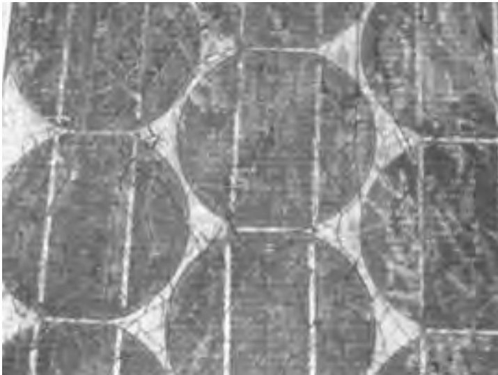
Figure 7.6: The effect of water and corrosion in a solar panel
